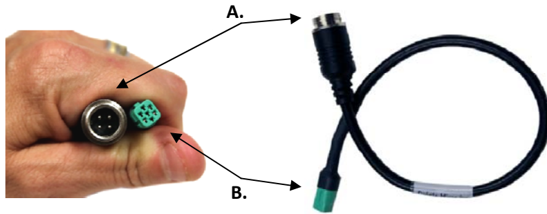
A. 7-pin Female Green Mini Amp Machine Connector B. 4-pin male OverView Connector
